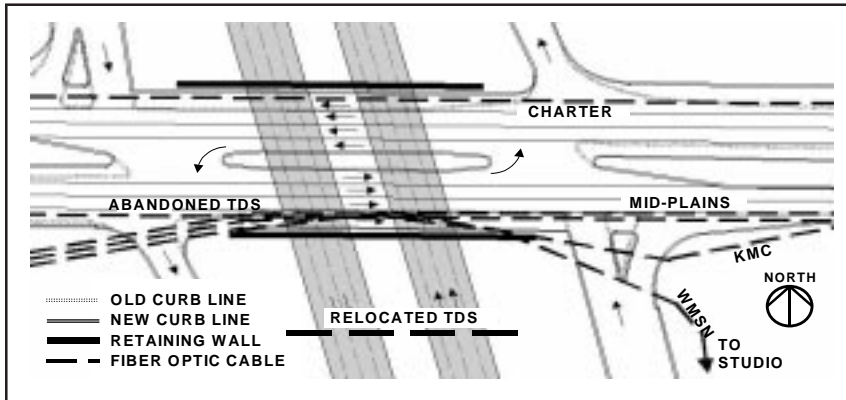
Figure 1. WISDOT Year 2000 Expansion Plan for the West Beltline interchange at Mineral Point Road. Five fiber optic cables cross the Beltline at this interchange. Drawing by the author based on WISDOT construction documents.
