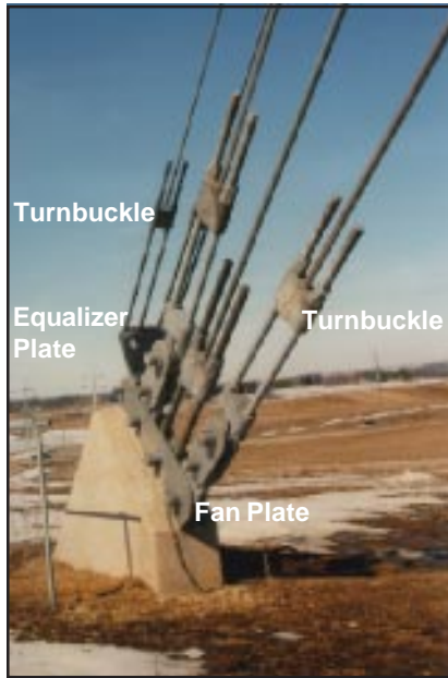
Figure 1. For a guyed tower, each anchor needs to be inspected.
